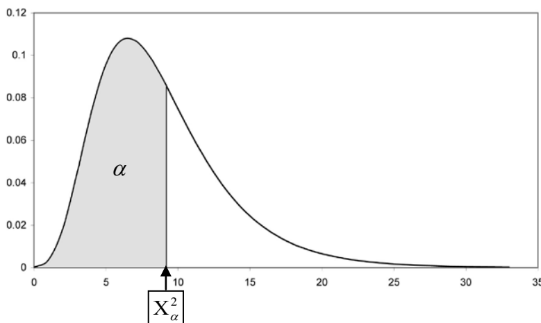
Figure 1: \chi^2 value calculated from the lower limit or the ( \alpha ) area to the left
