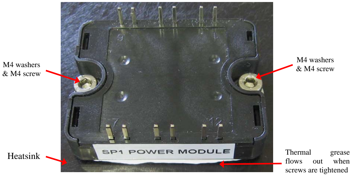
Fig 1: Proper application of thermal grease to the power module.
