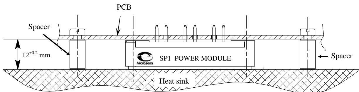
Fig 3: PCB onto the power module.
