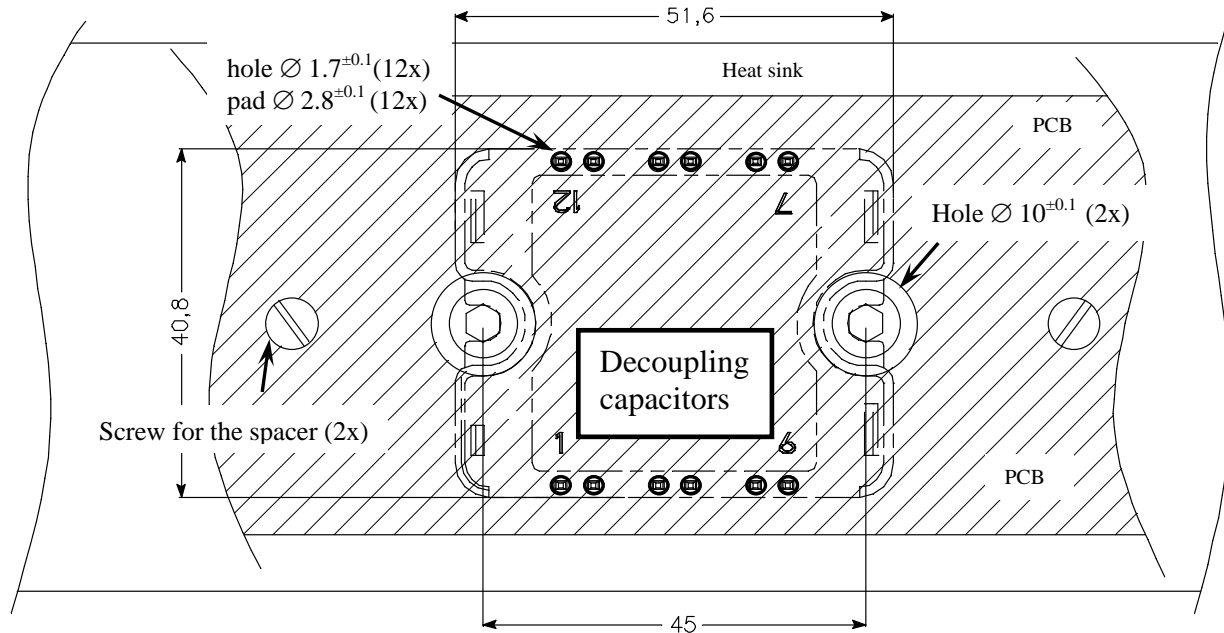
Fig 4: Pad and hole diameters (in millimeters) for a phase leg configuration.
